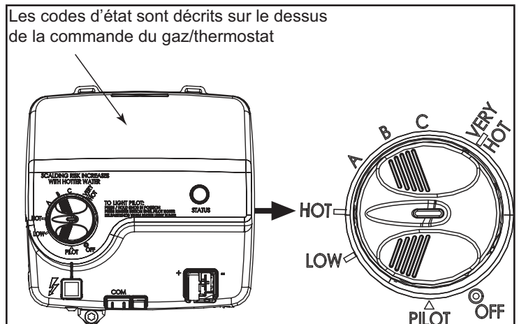
Figure 2D - Composantes d'installation.
