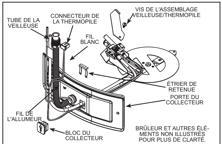
Figure 2C - Composantes d'installation.
