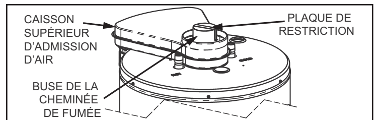
Figure 3O – Installation de la plaque de restriction
