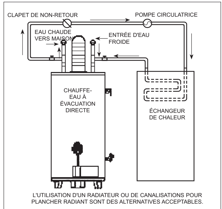
Figure 5 - Installation, chauffage combiné
